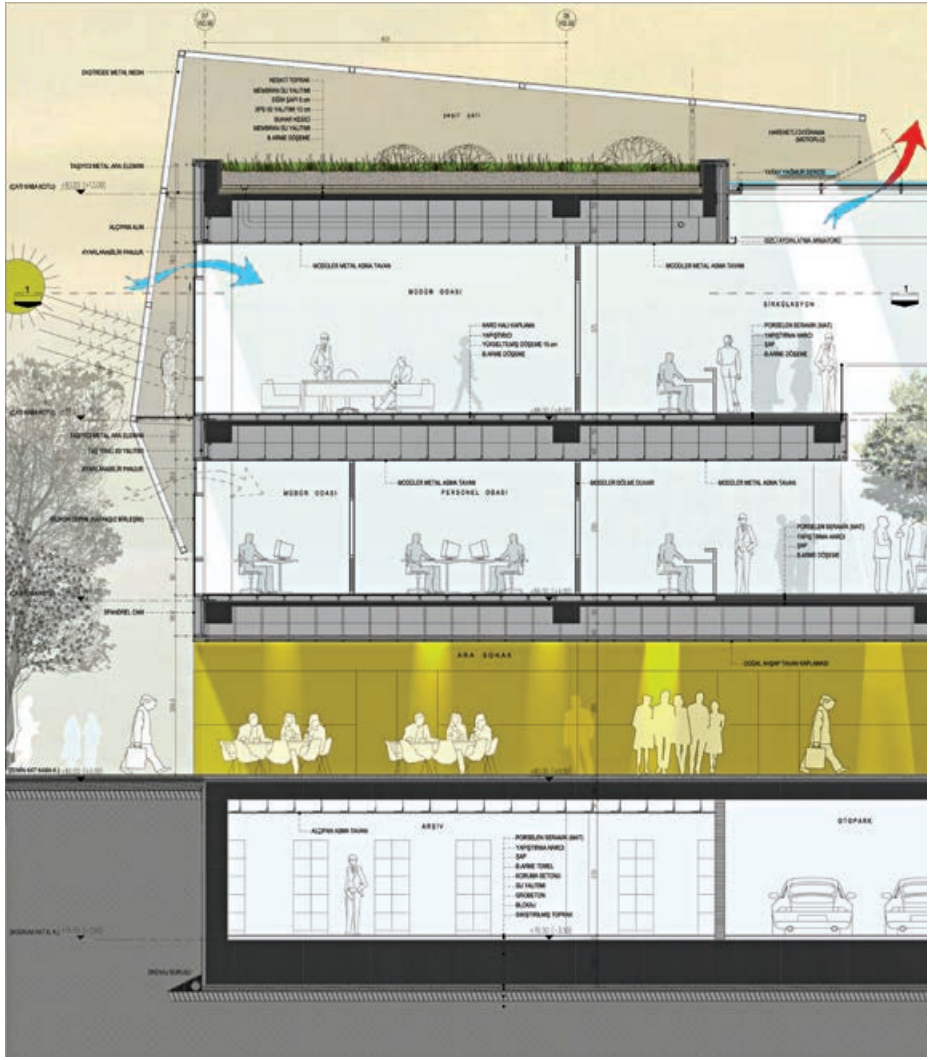
Sistem Kesiti Detail
